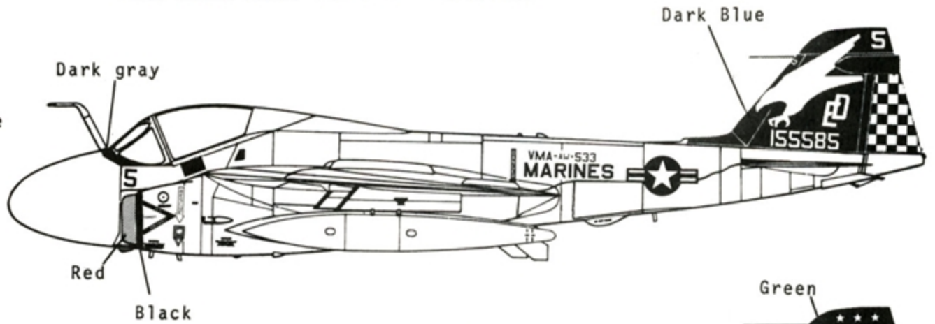
A-6A VMA-AW-533 Standard paint scheme
