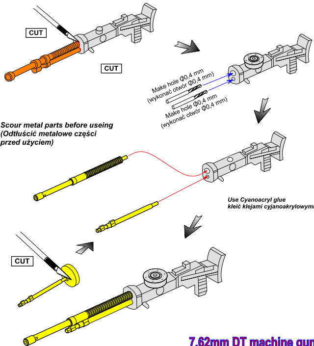
7,62mm DT machine gun
