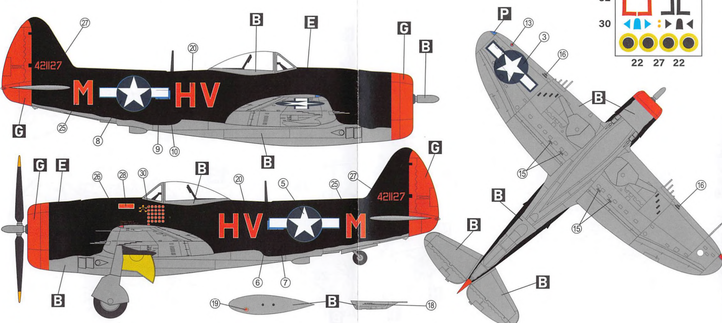
2 P-47M-1-RE, s/n 44-21127, Maj. Bolesław 'Mike' Gładych, 61st FS / 56th FG, Boxted, UK, 1945
