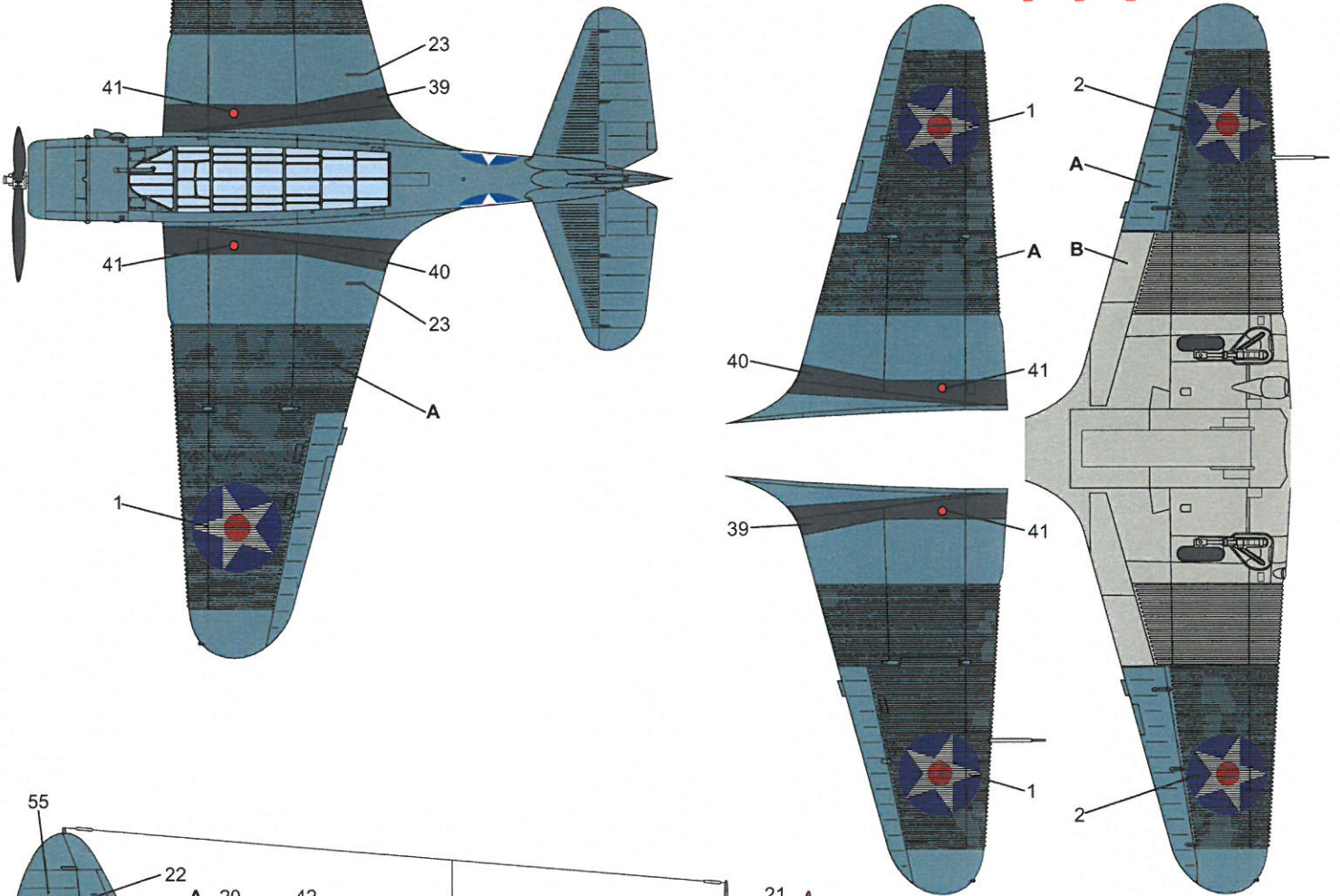
6 TBD-1, Bu.No. 0289, black 1, Lt Cdr E.E. Lindsey, VT-6, USS Enterprise (CV-6), 4 June 1942.
