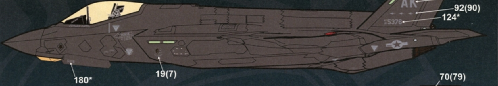
F-35A 19-5481 355TH FS EIELSON AFB, 2021
