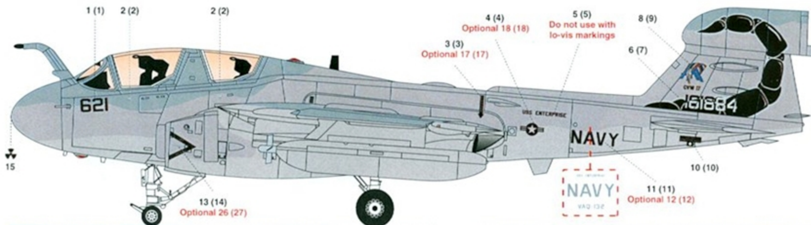
AIRCRAFT 1 • EA-6B BuNo. 161884 of CAG of VAQ-132 'Scorpions'. Standard FS 35237/36320/36375 Tactical Paint Scheme. Operation Southern Watch, Carrier Air Wing 17 on board USS Enterprise, Persian Gulf. Note aircraft also operated in slightly different lo-vis gray markings, use insignias 18, intake warnings 26 & 27, exhaust warnings 17 and fuselage markings 12 (replacing decals 5 and 11); eliminate decals 10.
