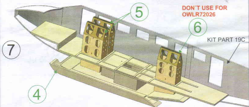
FRONT BOMBAY ASSEMBLY
