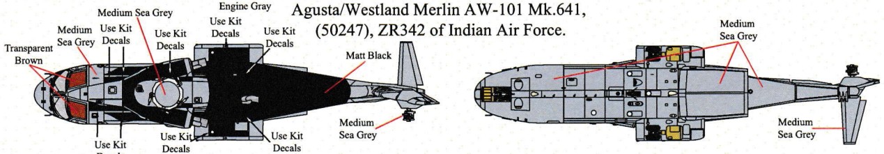
Agusta/Westland Merlin AW-101, Mk.610, (50231), ZR331, 'MS-21' Algerian Naval Forces.
